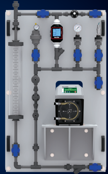
CFWS CHEM-FEED® Wall Mount Skid System
